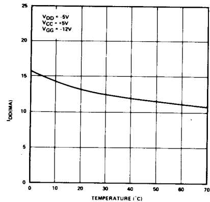
V DD POWER SUPPLY CURRENT VERSUS TEMPERATURE
